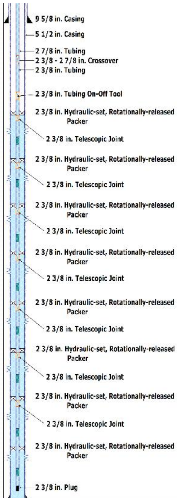
Fig. 9 – Hydraulic-Set Rotationally-Released Completion with Telescopic joints.
