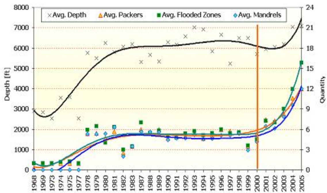
Fig. 3 – Injector-wells evolution.
