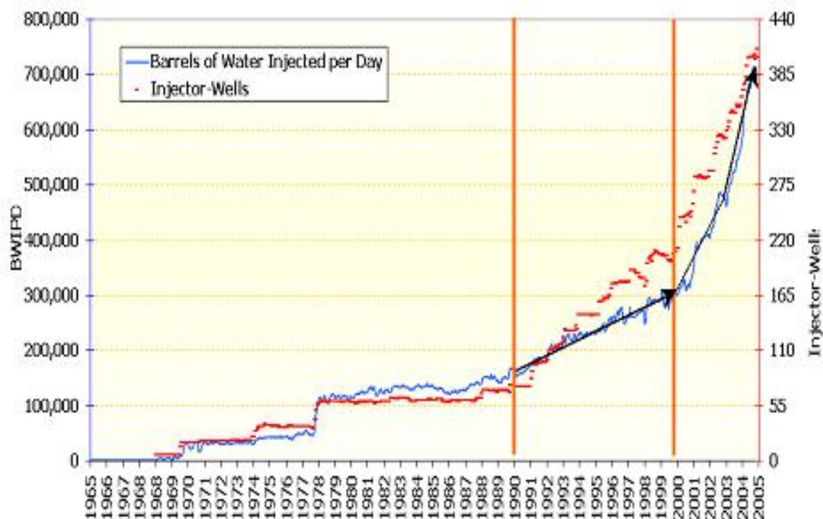
Fig. 2 – Waterflooding development.
