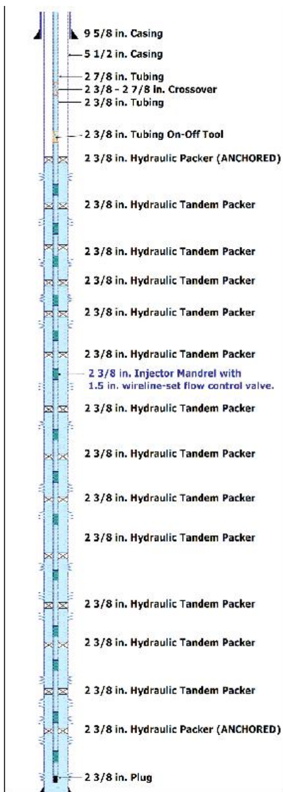
Fig. 6 – Hydraulic Packers Completion; 2 anchored points.
