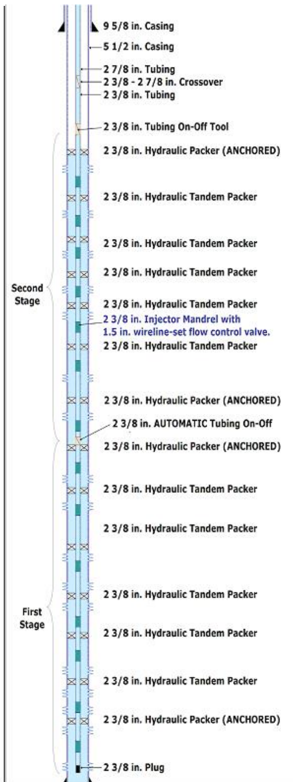
Fig. 7 – Hydraulic Packers Completion; anchored ends; 2 stages; 1 tubing run.
