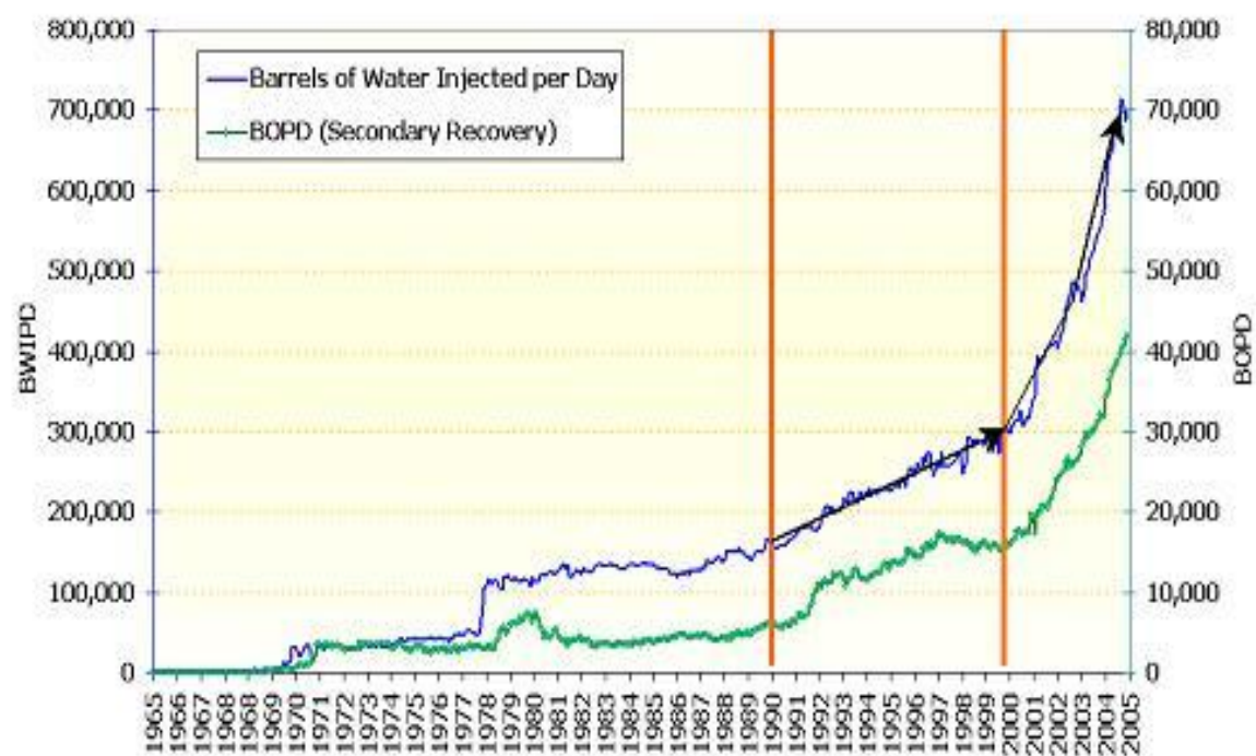
Fig. 1 – Injected water and secondary recovery oil production.
