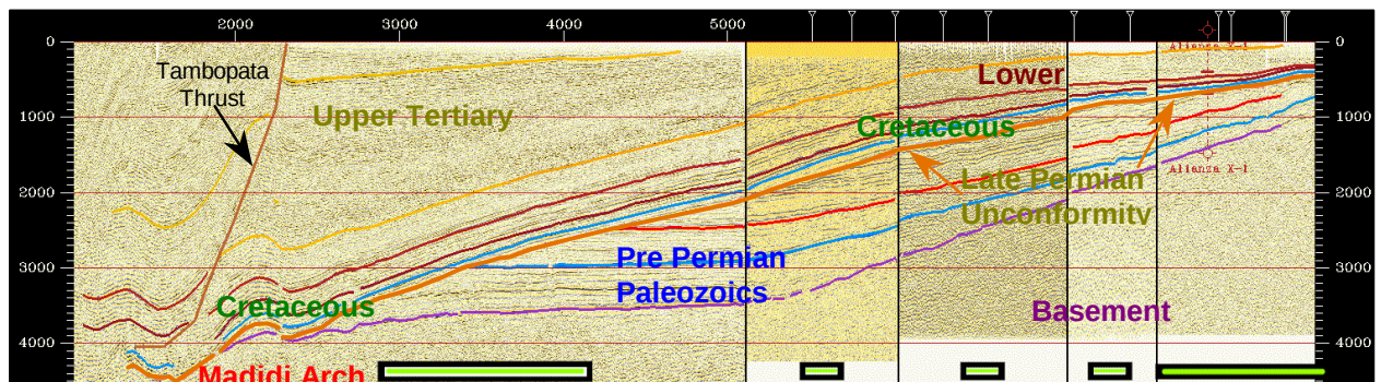
Figure 3. Regional seismic cross-section A-A' illustrating location of Madidi Arch relative to the frontal edge of the sub-Andean fold and thrust belt (Tambopata thrust fault).
