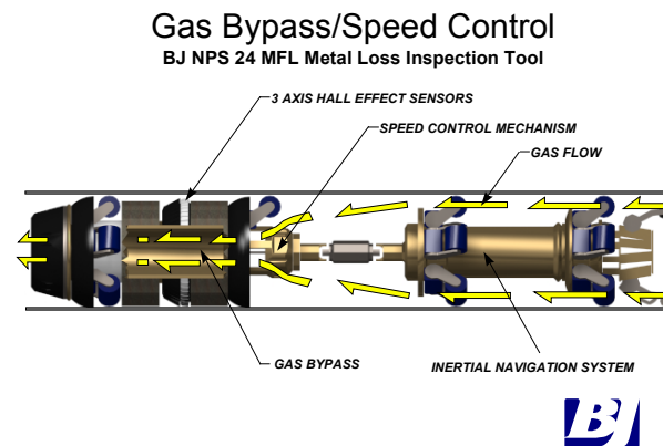
Figure 1. The Vectra MFL In-line Inspection Tool
