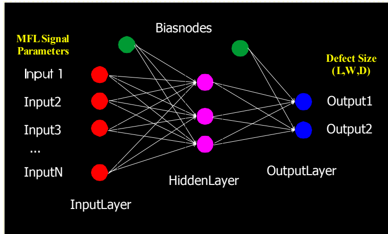
Figure 5. Schematic layout of a Neural Network
