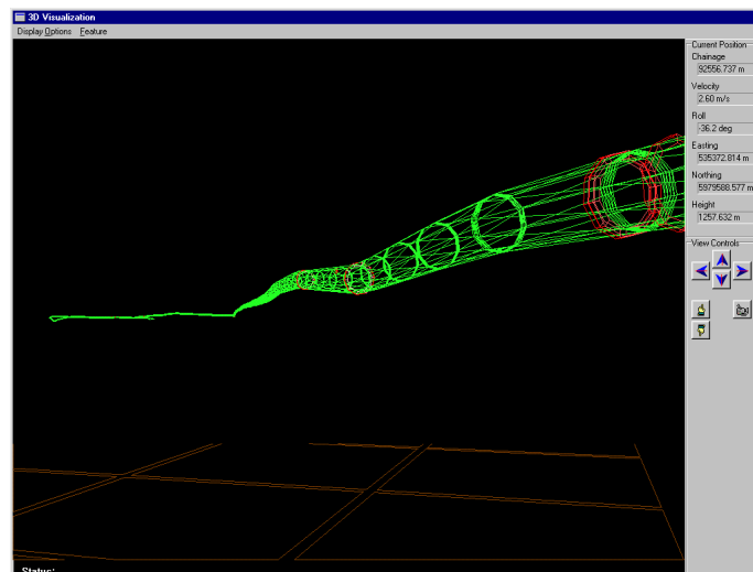
Figure 9. (a) The "Virtual Pipeline" generated from inertial data
