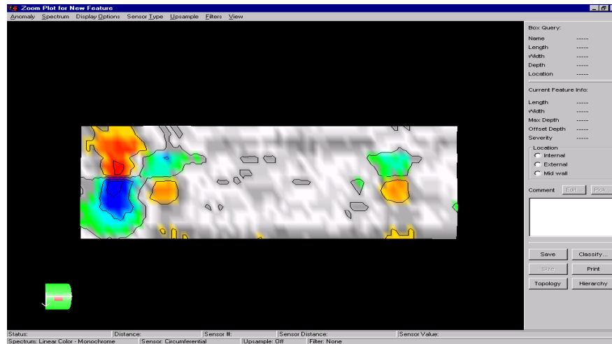
Figure 4 Use of the circumferential sensor to distinguish a long, narrow corrosion defect
