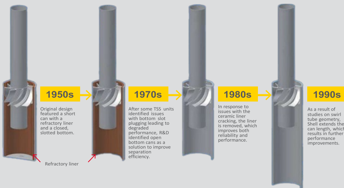
Figure 1: Swirl tube assembly development over the last 60+ years.
