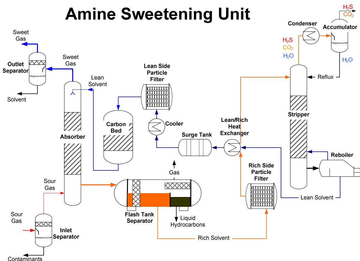
Figure 1. Amine System
