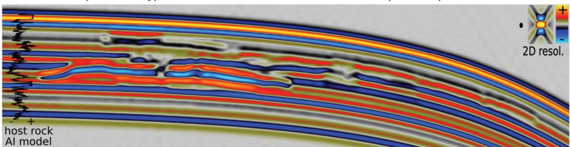
Figure 7. Seismic modelling results based on virtual outcrop models from El Manzano. a) We digitally interpreted the kilometer-scale virtual model to extract detailed geometries of the intrusive bodies. We then superimposed the outcrop-based sill intrusions on a host rock model and generated synthetic seismic sections at c. 25 Hz resolution for three modelling cases: b) homogenous siliciclastic host, c) Norwegian margin type layered siliciclastic host with low acoustic impedance, and d) Neuquén Basin type host including shales, carbonates, and gypsum of the Mendoza Group.
