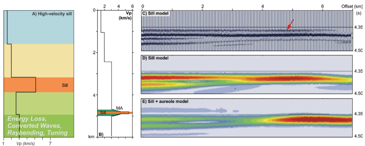
Figure 8. Aspects related to seismic imaging of sill intrusions. a) Schematic Earth model of a high-velocity sill intrusion in the sedimentary basin. b) Velocity model of an intruded basin simplified from observations in the Vøring Basin used for synthetic seismic modeling in c to e. c) Flattened seismic gather for model without a MA. d) Flattened instantaneous amplitude in model without MA; red shows high amplitudes. e) Flattened instantaneous amplitude in model with a MA; red shows high amplitudes. MA: Metamorphic velocity aureole. See Planke et al. (2015) for modeling details.
