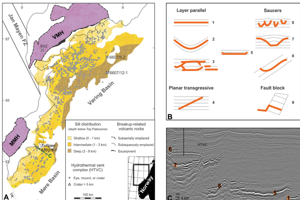
Figure 4. Distribution and seismic characteristics of intrusive complexes on the mid-Norwegian continental margin. a) Distribution of lava, sills, and hydrothermal vent complexes in the Vøring and Møre basins. Key igneous wells are also located. b) Characteristic geometries of sill reflections. c) Seismic profile showing high-amplitude sill reflections in the Møre Basin. Numbers represent geometries shown in Figure 4b. A and b modified from Planke et al. (2005).
