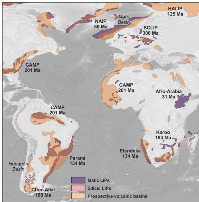
Figure 2. Distribution of large igneous provinces (LIPs) and prospective volcanic basins system in the Atlantic region where both syn- and post-magmatic influences comprise important elements of the petroleum system are highlighted. LIPs modified after Bryan and Ferrari (2013).
