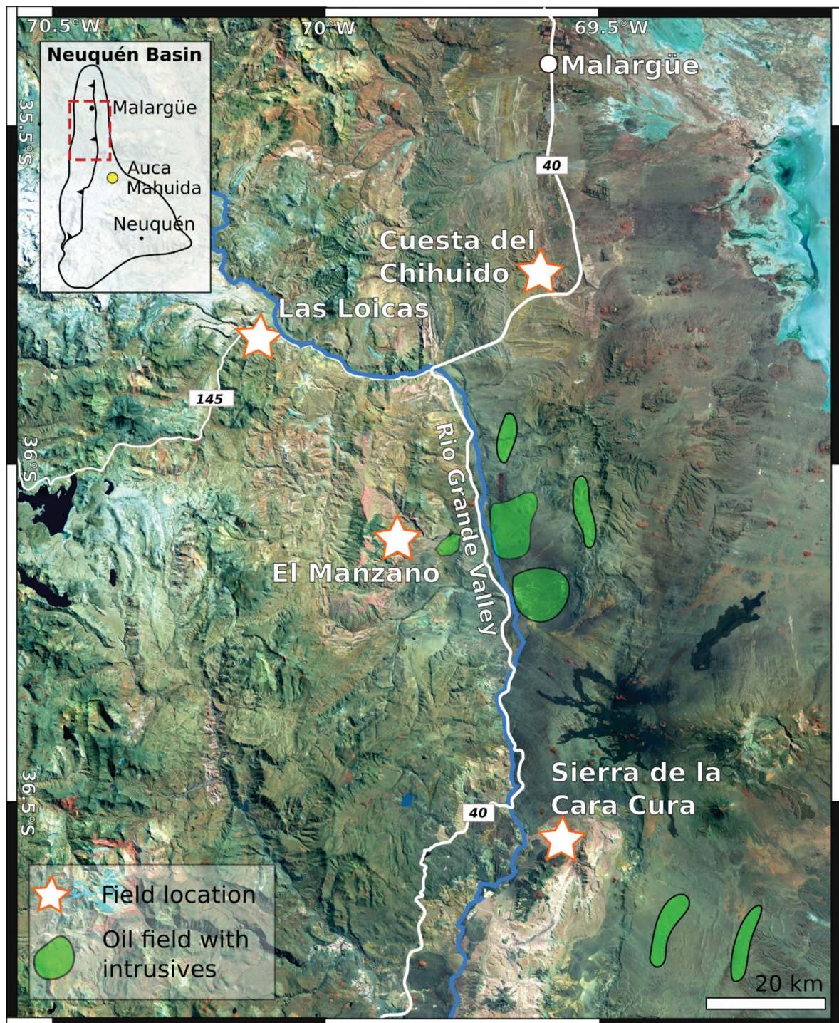
Figure 3. Map showing the Neuquén Basin study area south of Malargüe, Argentina. The stars indicate main outcrop localities of igneous sills, which we used as analogues to subsurface sill complexes. Note in particular the close proximity of the El Manzano outcrop to several oil fields in the Rio Grande valley, where the direct subsurface analogues are producing from igneous reservoirs. Landsat satellite image.
