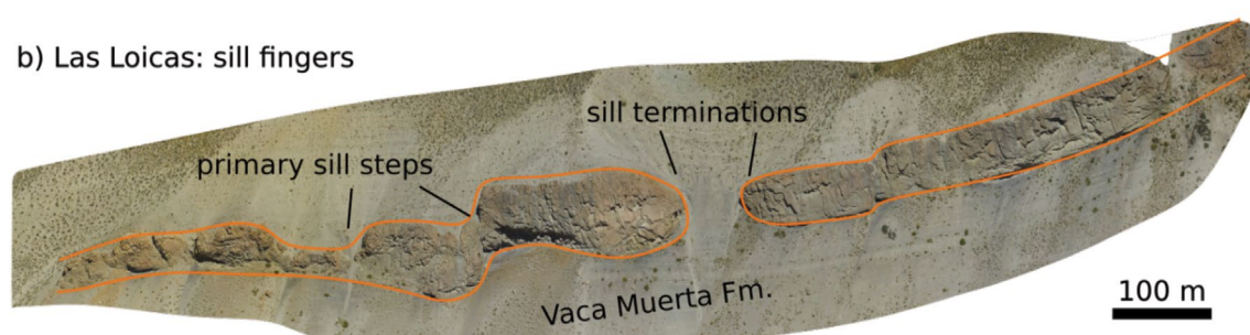
Figure 6. Examples of outcropping intrusions from a) El Manzano and b) Las Loicas, with sills emplaced in the Agrio and Vaca Muerta formations, respectively (sills between orange lines). We captured both outcrops using drone-based photogrammetry surveys. The kilometer-scale sill complex exposed at El Manzano was digitally mapped and used as structural input for the seismic modelling presented in Figure 7.
