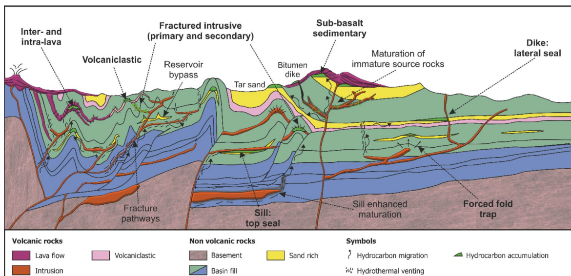
Figure 10. Conceptual model of a compressional margin setting with volcanic associated petroleum system influences annotated. The tectonic structure is broadly based on an E-W cross section through the Neuquén Basin, after Uliana and Legarreta (1993), but the annotated features bear no geographical relation to the section and are generic to compressional margins.
