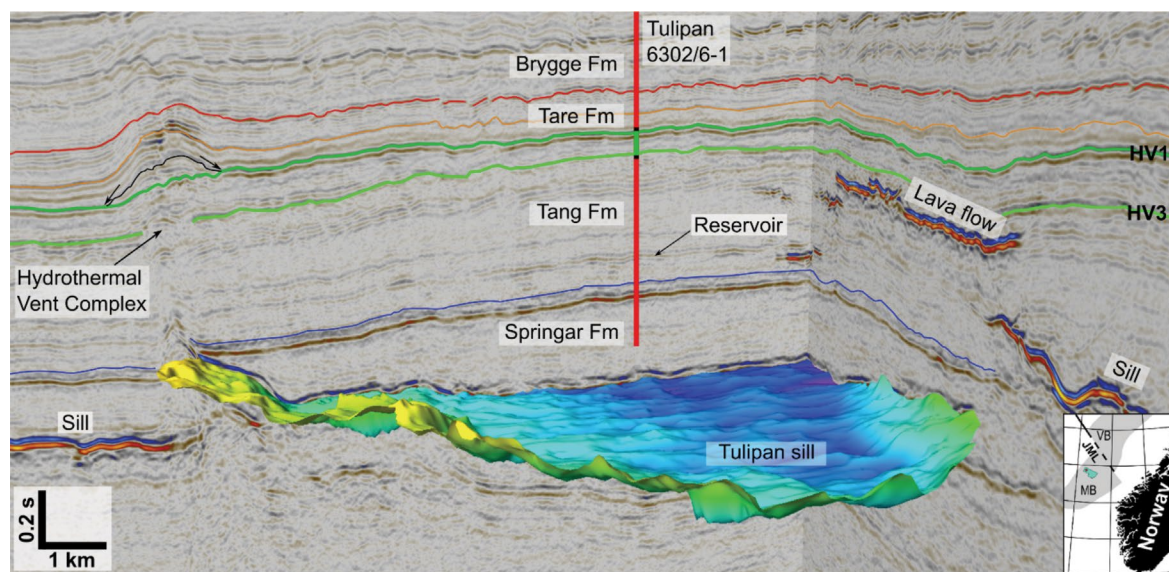
Figure 5. Three-dimensional image of the Tulipan saucer-shaped sill and overlying forced fold in the Møre Basin (Figure 3). A small gas discovery in Paleocene sandstones of the Tang Fm. was proven by well 6302/6-1. The paleosurface is located near the HV3 horizon. Modified from Kjøberg et al. (2017).
