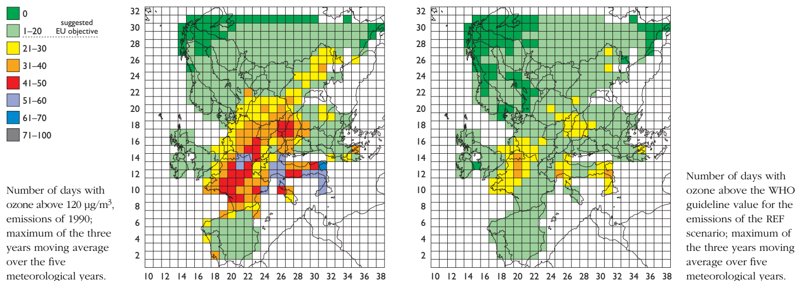
FIGURE 2: NUMBER OF DAYS WITH OZONE ABOVE 120 \mu\text{g}/\text{m}^3 (left: 1990 emissions; right: 2010 REF scenario)
