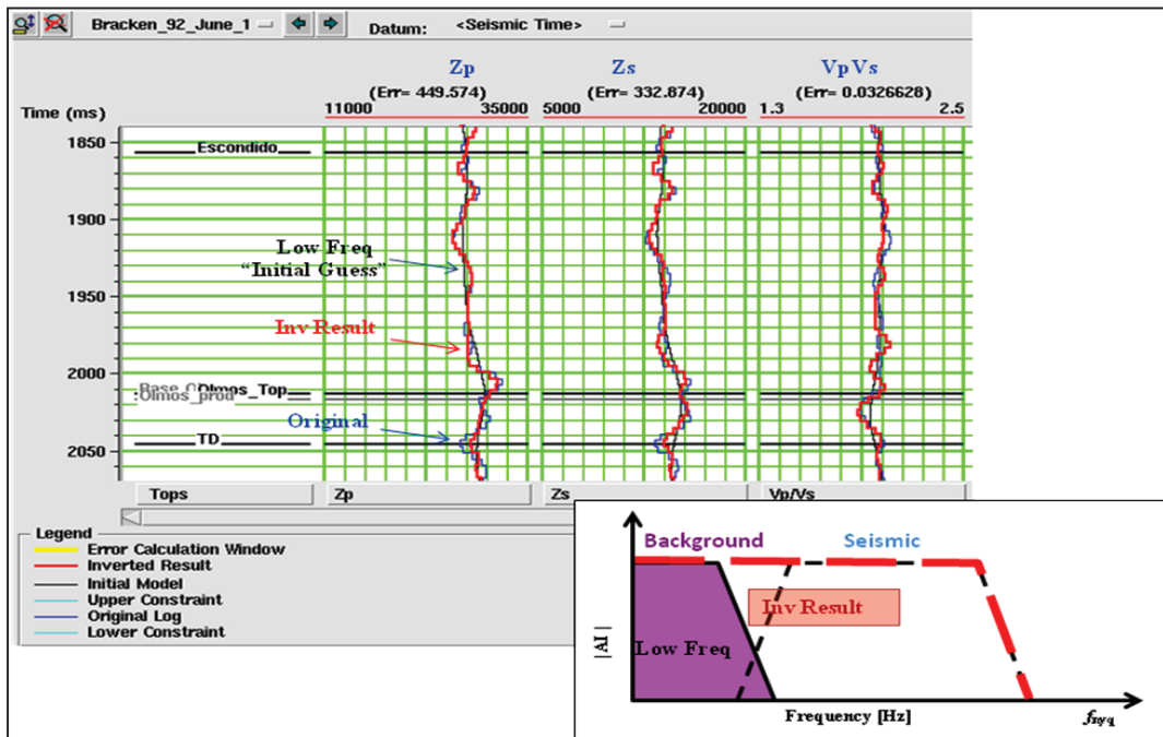
Figure 10. Upper figure shows the original (blue), the filtered log (black), and the inverted result (red) for the P and S-Impedance and V_p/V_s ratio at one of the well locations. Lower figure shows the frequency spectra for each log curve. Note that by filtering back the original well log the low frequencies can be recovered.
