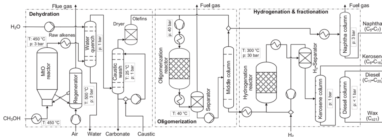
Fig 11: Proceso MtJ. Fuente: Sustainable synthetic carbon-based fuels for transport. 2019. The Royal Society.
