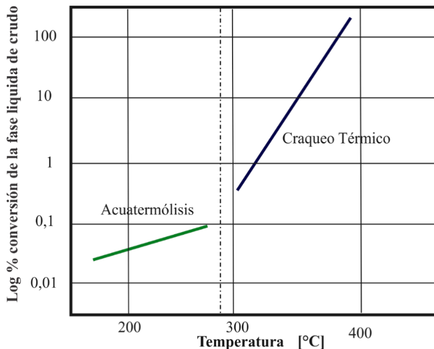
Fig. 2 - Conversion de la fase líquida de hidrocarburos en las reacciones ocurridas en sistemas aguas aceite. Adaptado: Hyne, J. B. (1986). Aquathermolysis : a synopsis of work on the chemical reaction between water (steam) and heavy oil sands during simulated steam stimulation. AOSTRA Publication Series, (no 50), 55, [27] leaves.
