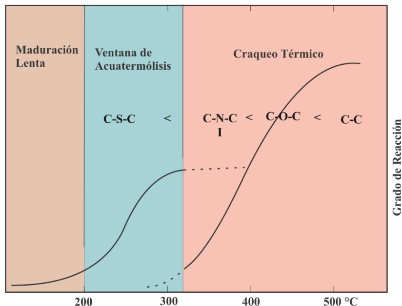
Fig. 1 -Ventana de ocurrencia para las reacciones de acuatermolisis. Adaptado de: Hyne, J. B. (1986). Aquathermolysis : a synopsis of work on the chemical reaction between water (steam) and heavy oil sands during simulated steam stimulation. AOSTRA Publication Series, (no 50), 55, [27] leaves.
