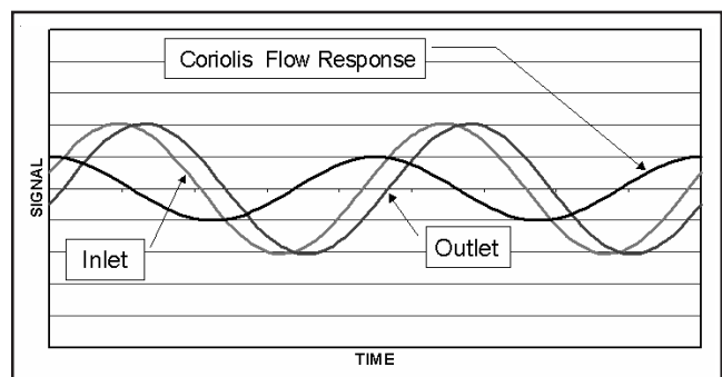
Figure 10 – Coriolis Response Signal
