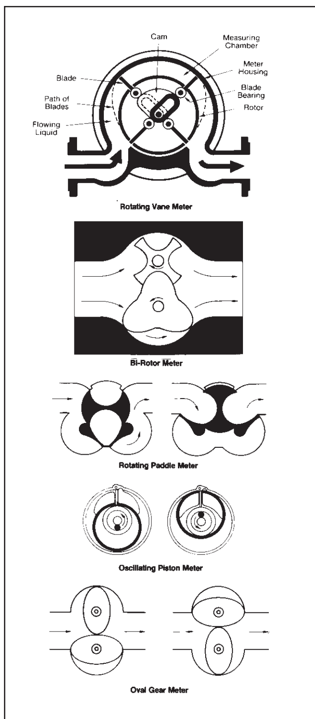
Figure 1 — PD Meter Types
