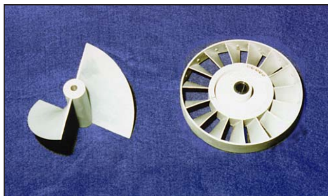
Figure 5 – Helical vs. Conventional Turbine Meter Rotors
