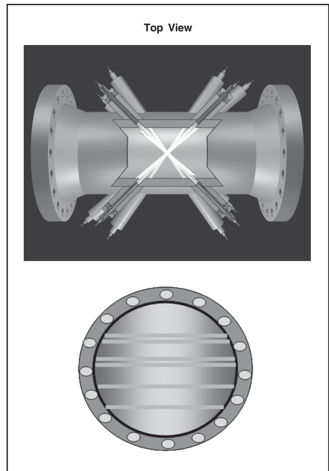
Figure 12 – Multipath Ultrasonic Meter
