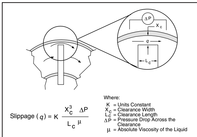
Figure 2 — Slippage across meter clearances
