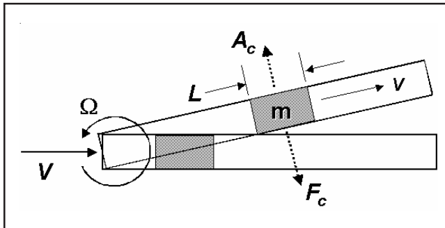
Figure 7 – Fluid Moving Through the Meter Tube
