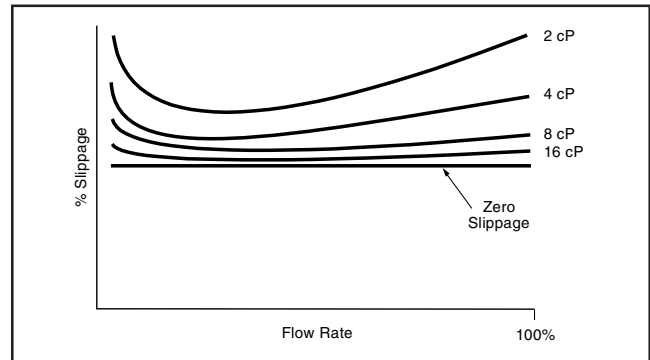
Figure 3 — Effect of Viscosity on PD measurement range
