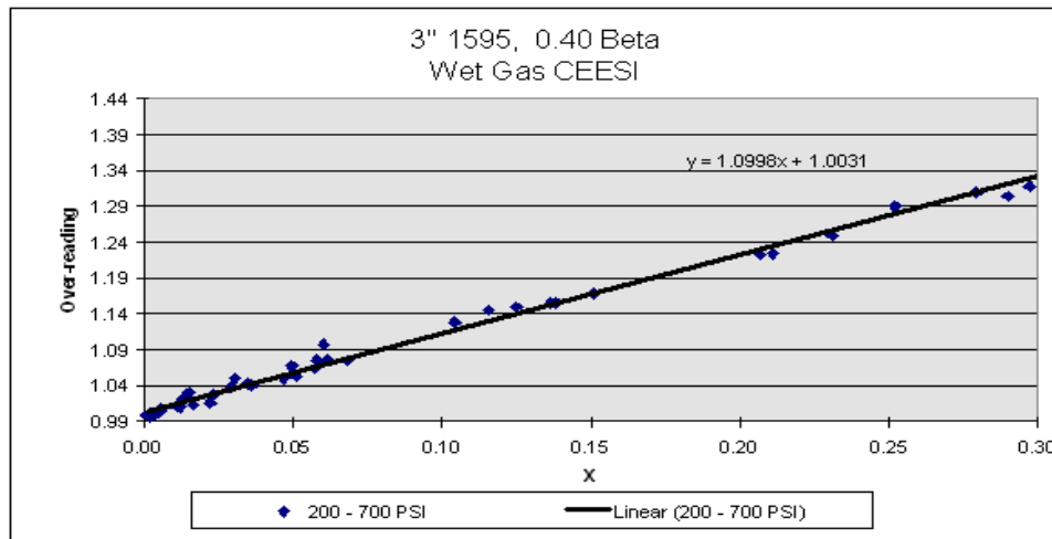
Figure 9 Model 1595 over-reading vs. Lockhart-Martinelli 0.4 Beta, with curve fit
