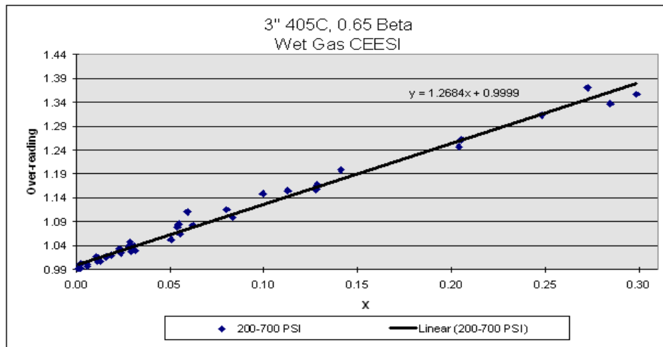
Figure 12 Model 405C over-reading vs. Lockhart-Martinelli 0.65 Beta with curve fit
