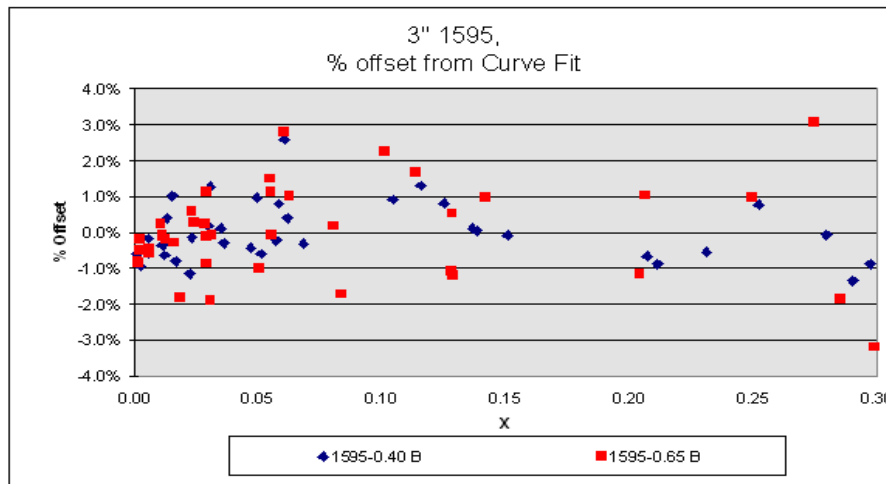
Figure 13 Model 1595 Calculate offset from measured vs. Lockhart-Martinelli Number
