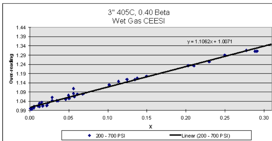
Figure 11 Model 405C over-reading vs. Lockhart-Martinelli 0.40 Beta with curve fit
