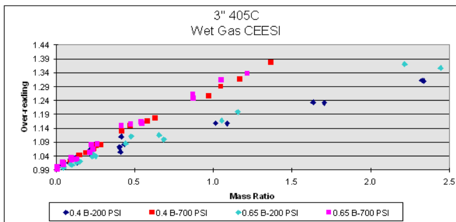
Figure 6 Model 405C over-reading vs. Mass Ratio
