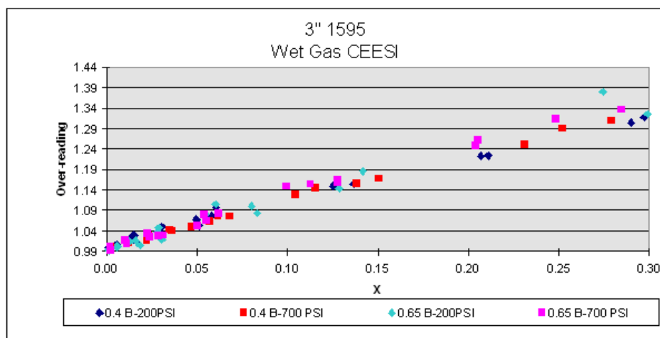
Figure 7 Model 1595 over-reading vs. Lockhart-Martinelli Number
