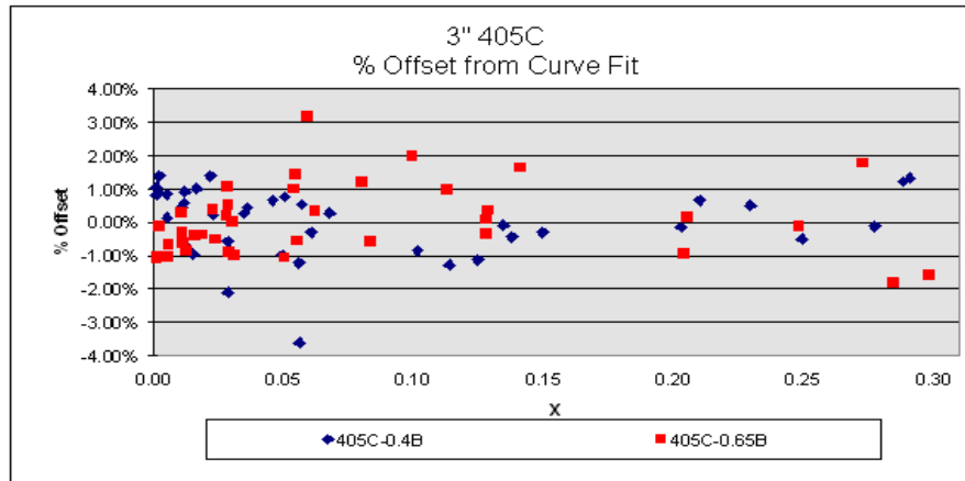
Figure 14 Model 405C Calculated offset from measured vs. Lockhart-Martinelli Number
