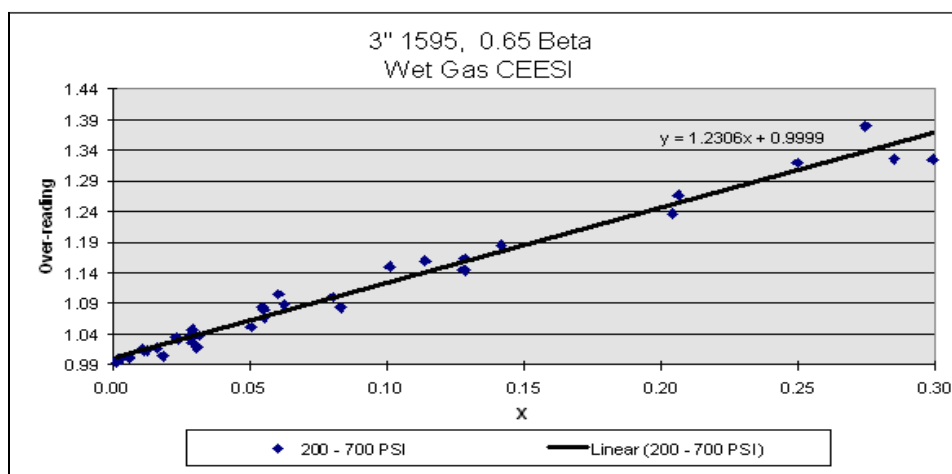
Figure 10 Model 1595 over-reading vs. Lockhart-Martinelli 0.65 Beta with curve fit
