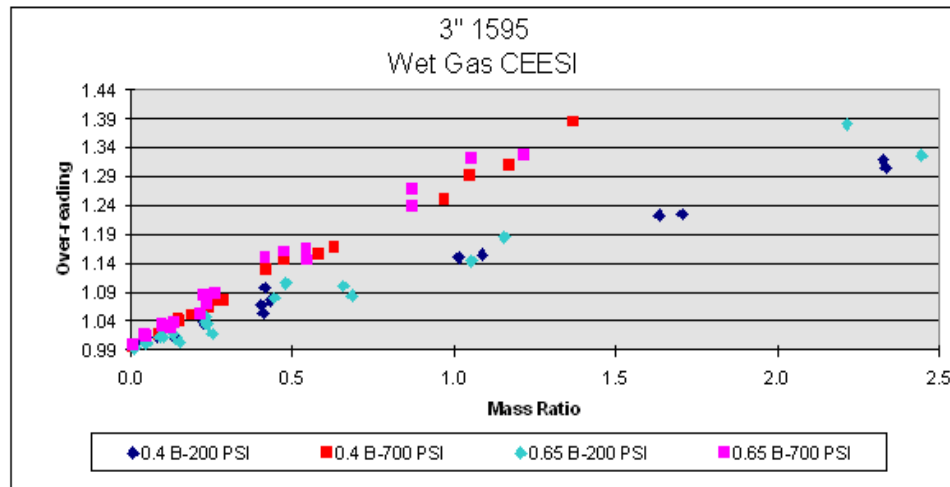
Figure 5 Model 1595 over-reading vs. Mass Ratio
