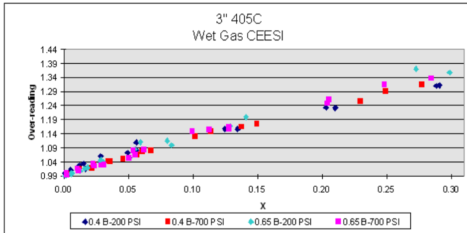
Figure 8 Model 405C over-reading vs. Lockhart-Martinelli
