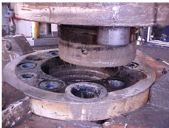
Figure 4. Riser Flange
